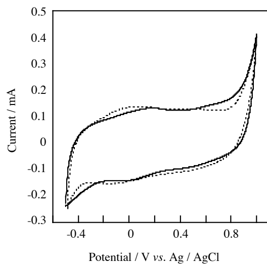
Supplementary Fig. 2 Comparison of CV patterns after 100 redox cycles: SWNTs•DNA/poly(EDOT) composite film (solid line), poly(EDOT) film (dashed line).
